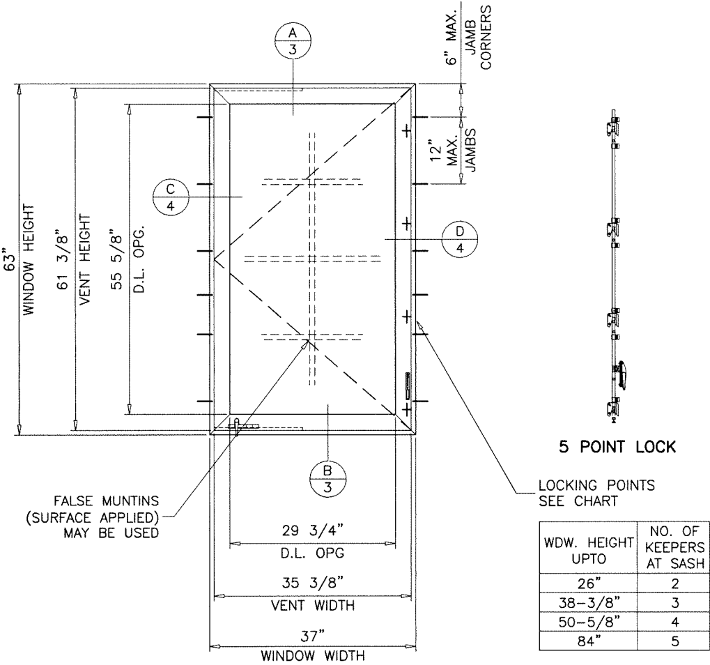
TYPICAL ELEVATION TESTED UNIT
